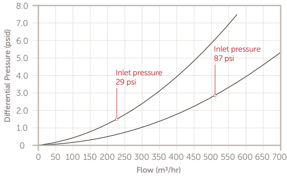
Savana 20" Cartridges
