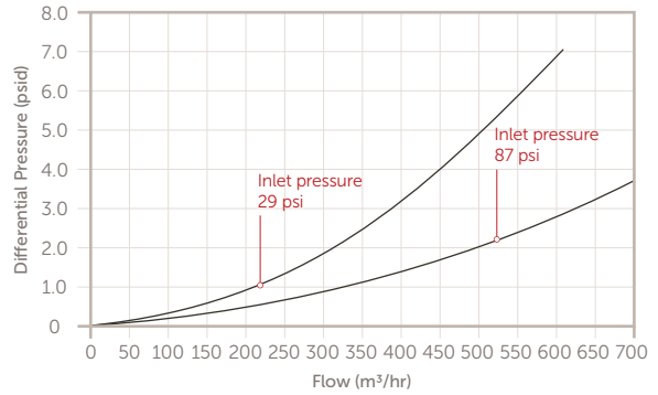
Savana 30" Cartridges
